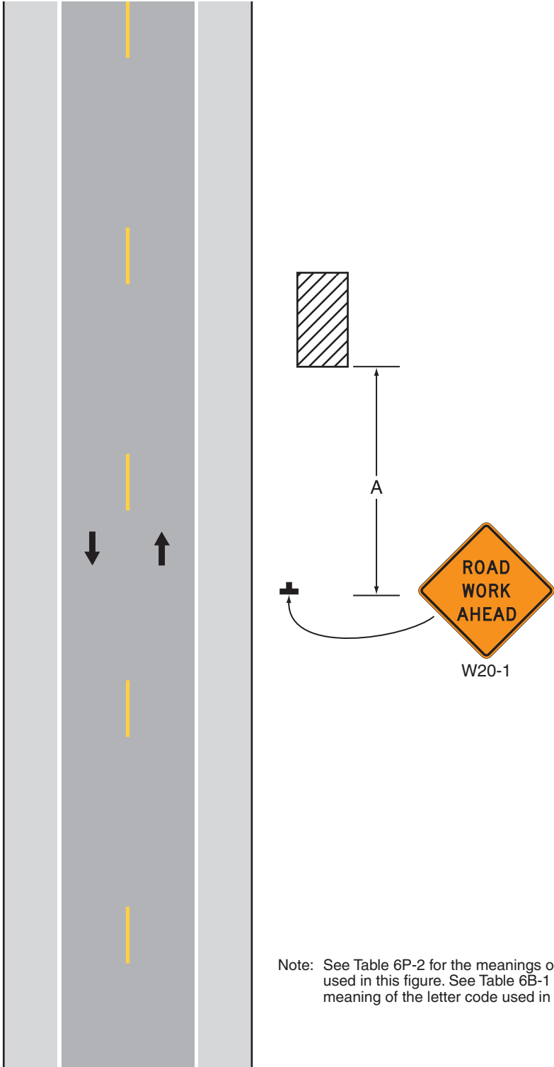
Typical Application 1
