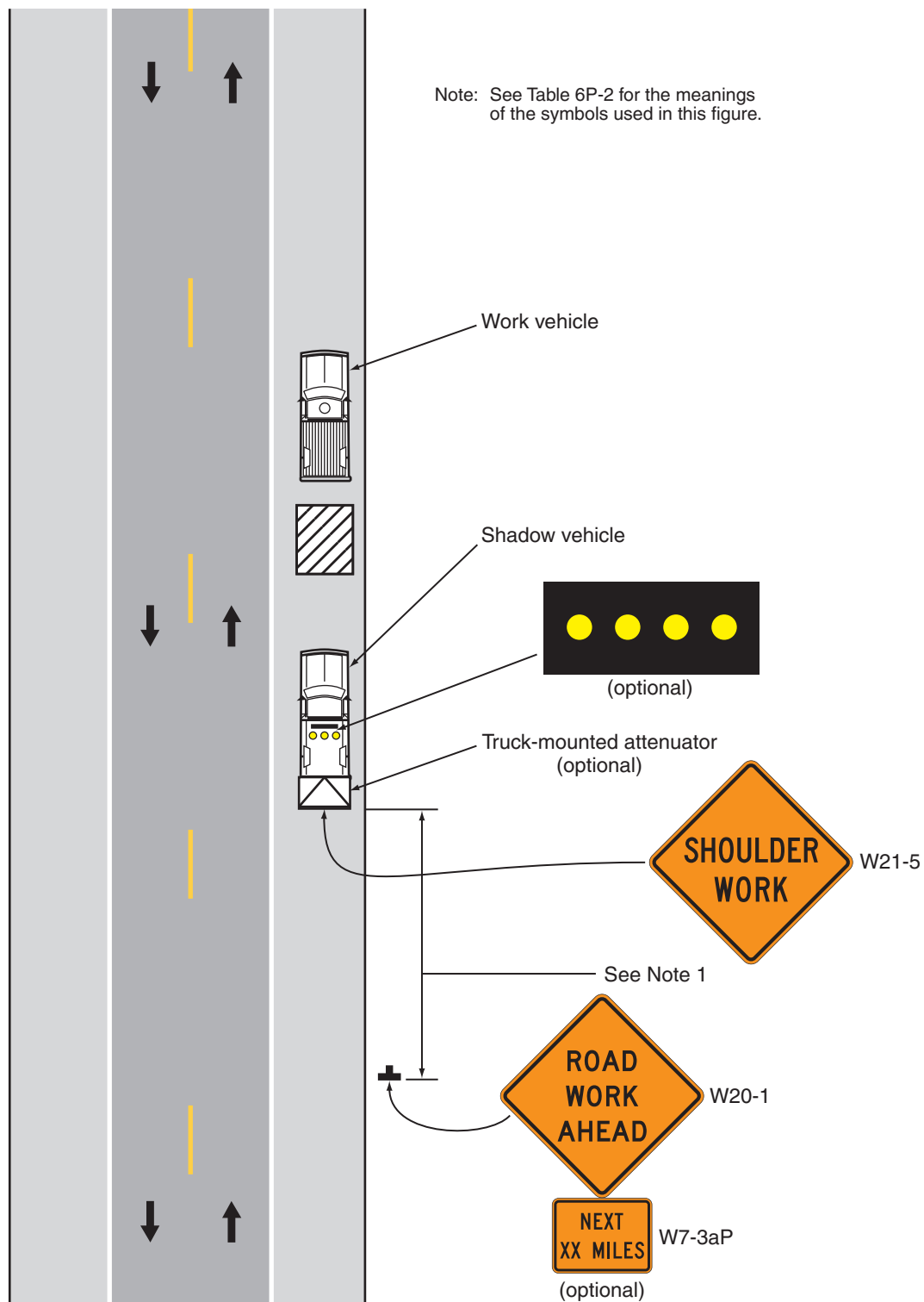
Typical Application 4
