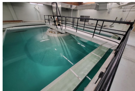
Softening Clarifier at ELMWSA
